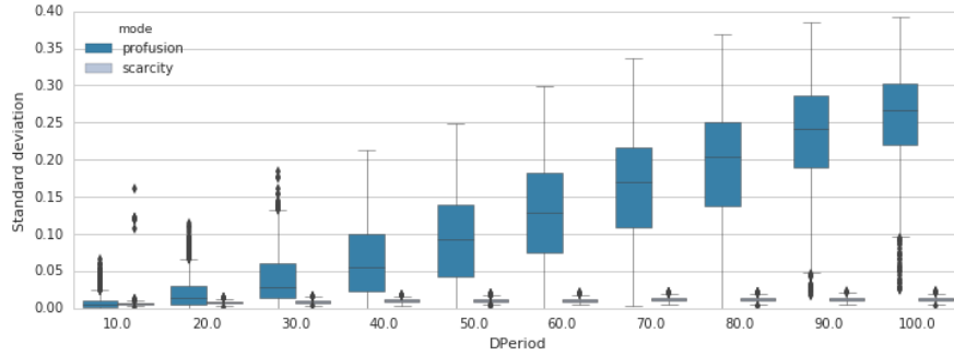
Fig. 4: Profusion vs Scarcity - Mean Standard deviation of Number of Stifiers at the convergence computed over 10 experiments for each initial infected node with the same diffusion parameters.
