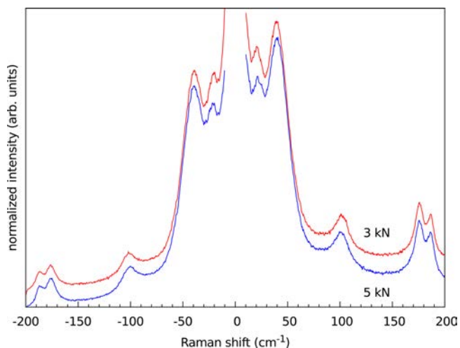
Figure 7. LFR spectra of ZrO 2 NPs sintered at 400 °C with an applied force of 3 (top) and 5 kN (bottom). The spectra are vertically shifted for clarity.
