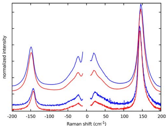
Figure 6. Normalized LFR spectra at room temperature (2 top spectra) and T \approx 100 K (2 bottom spectra) of TiO 2 NPs compacted (blue) and sintered at 300 °C (red). The spectra are vertically shifted for clarity.
