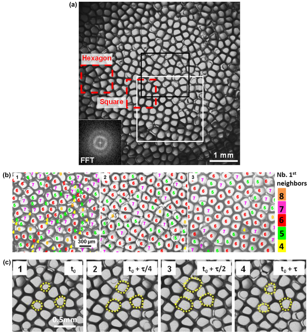
FIG. 3. (a) Global view of the interface at t = 13.9 h ( L = 50 mm), for V = 1 \mu\text{m/s} and G_1 = 19 \text{ K/cm} , with the corresponding FFT image highlighting the high spatial array disorder. (b) Enlarged view of first neighbors in the area marked with a white square in (a) at different times: 1.5 h (5.4 mm), 6.7 h (24.1 mm), and 14.1 h (50.8 mm). (c) Enlarged view of area marked with a black square in (a) at different times t_0 = 14.3 h, t_0 + \tau/4 = 14.6 h, t_0 + \tau/2 = 14.8 h, and t_0 + \tau = 15.1 h (oscillation period \tau = 48 min).
