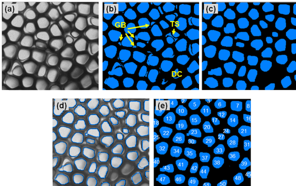
FIG. 1. (a) Example of an initial raw image ( 3.2 \times 3.2 mm 2 ). (b) Binary image evidencing some defects resulting from dark cells (DC), tip-splitting events (TS), or groove bottoms (GB). (c) Binary image after processing with “opening function”. (d) Contours of apparent cell area on corrected binary image superimposed on the initial raw image. (e) Tagged binary image ( V = 1 \mu\text{m/s} , G_1 = 19 K/cm).
