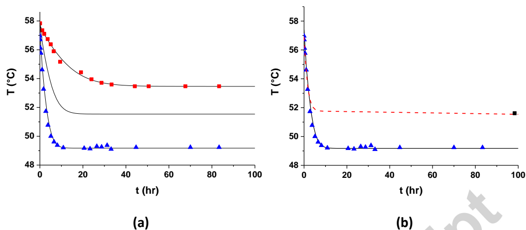
Figure 3 – (a) Interface temperature ( T ) as function of time ( t ) for different SCN-camphor alloys (■, 0.24 wt%, 0.30 \mu\text{m/s} and 6.0 K/mm; ◆, 0.5 wt%, 0.38 \mu\text{m/s} and 6.6 °C/mm; ▲, 0.9 wt%, 0.42 \mu\text{m/s} and 9.8 K/mm). The experimental results are compared to KRFT [26] model results (–) with \Delta \rightarrow \infty . (b) Interface temperature as function of time for SCN-0.9wt% camphor: ▲, this work; ■, TL [11] and KRFT model results. The solid line corresponds to \Delta = 10 that fit our data, and the dotted line is for \Delta = 2 that gives the interface temperature at long time that corresponds to the interface temperature value reported by TL [11].
