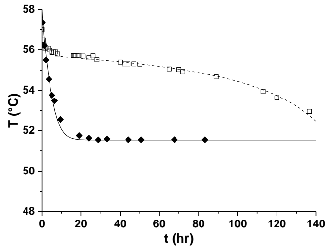
Figure 4 – Interface temperature for the SCN - 0.5 wt% camphor alloy as a function of time for different experimental conditions: □, V = 0.1 \mu\text{m/s} and G = 7.1 \text{ }^\circ\text{C/cm} ; and ◆, V = 0.38 \mu\text{m/s} and G = 6.6 \text{ }^\circ\text{C/mm} . The experimental results are compared to KRFT [26] model results with \Delta = 2 (--) and \Delta \rightarrow \infty (-).
