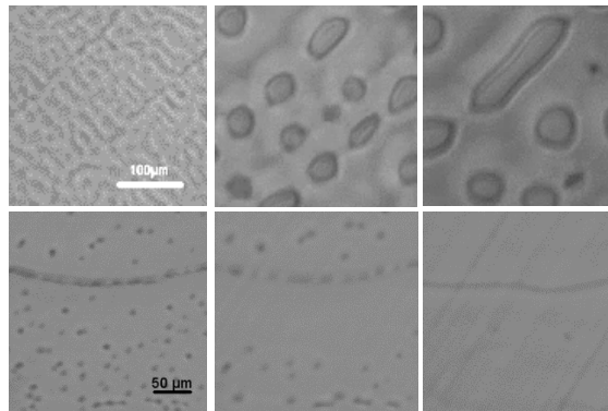
Figure 5 – Light microscopy images of the evolution of SCN-3 wt% camphor (a,b,c) and 1.5 wt% camphor (d,e,f) under isothermal conditions (38 °C) as a function of time (t).
