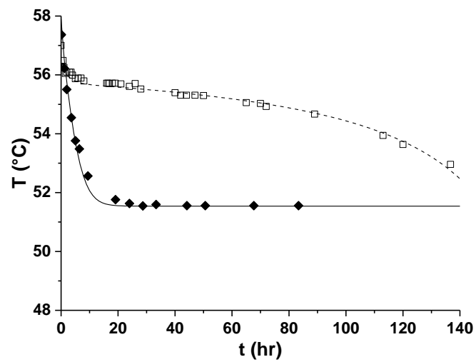
Figure 4 – Interface temperature for the SCN - 0.5 wt% camphor alloy as a function of time for different experimental conditions: □, V = 0.1 \mu\text{m/s} and G = 7.1 \text{ }^\circ\text{C/cm} ; and ◆, V = 0.38 \mu\text{m/s} and G = 6.6 \text{ }^\circ\text{C/mm} . The experimental results are compared to KRFT [26] model results with \Delta = 2 (--) and \Delta \rightarrow \infty (-).
