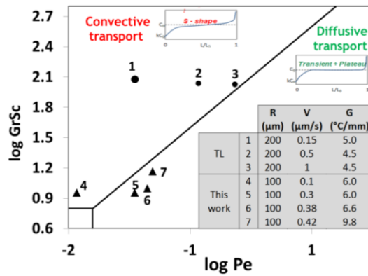
Figure 2 – Grashof-Schmidt number versus Peclet number diagram [16, 17] showing the regions of diffusive and convective growth. Experimental conditions used by TL [11] and those used in this work are shown in the inset table.
