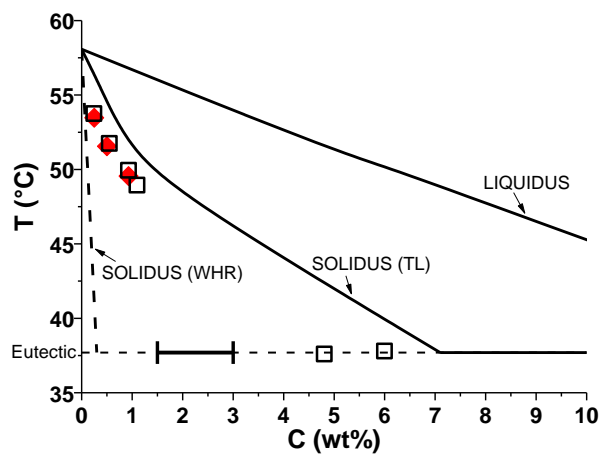
Figure 1 – Phase equilibria data for the binary alloy SCN-camphor: \blacklozenge , directional solidification measurements; \square , DSC measurements; —, TL [11]; - -, WHR [14]. The segment ( )—( ) represents the range where the solubility limit must be as determined by isothermal annealing.
