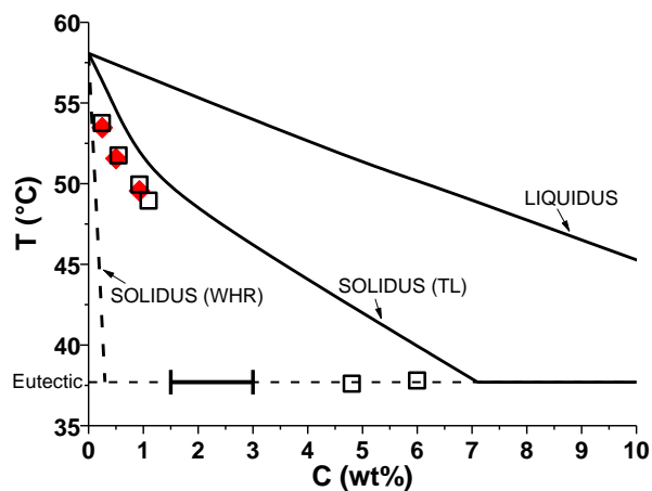
Figure 1 – Phase equilibria data for the binary alloy SCN-camphor: ♦, directional solidification measurements; □, DSC measurements; —, TL [11]; - -, WHR [14]. The segment ( )—( ) represents the range where the solubility limit must be as determined by isothermal annealing.
