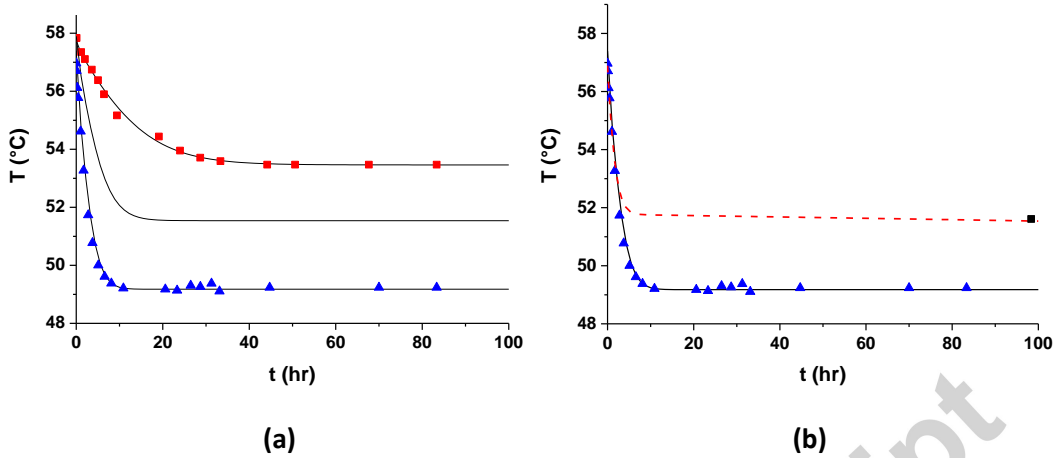
Figure 3 – (a) Interface temperature ( T ) as function of time ( t ) for different SCN-camphor alloys (■, 0.24 wt%, 0.30 \mu\text{m/s} and 6.0 K/mm; ◇, 0.5 wt%, 0.38 \mu\text{m/s} and 6.6 ^{\circ}\text{C/mm} ; ▲, 0.9 wt%, 0.42 \mu\text{m/s} and 9.8 K/mm). The experimental results are compared to KRFT [26] model results (–) with \Delta \rightarrow \infty . (b) Interface temperature as function of time for SCN-0.9wt% camphor: ▲, this work; ■, TL [11] and KRFT model results. The solid line corresponds to \Delta = 10 that fit our data, and the dotted line is for \Delta = 2 that gives the interface temperature at long time that corresponds to the interface temperature value reported by TL [11].
