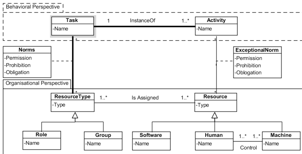
Fig. 3. organisational perspective
