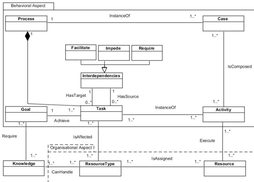
Fig. 2. behavioral perspective
