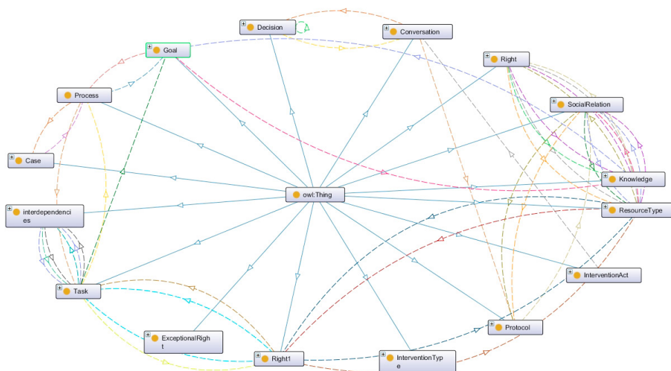
Fig. 6. Hierarchy of schema graph of our ontology
