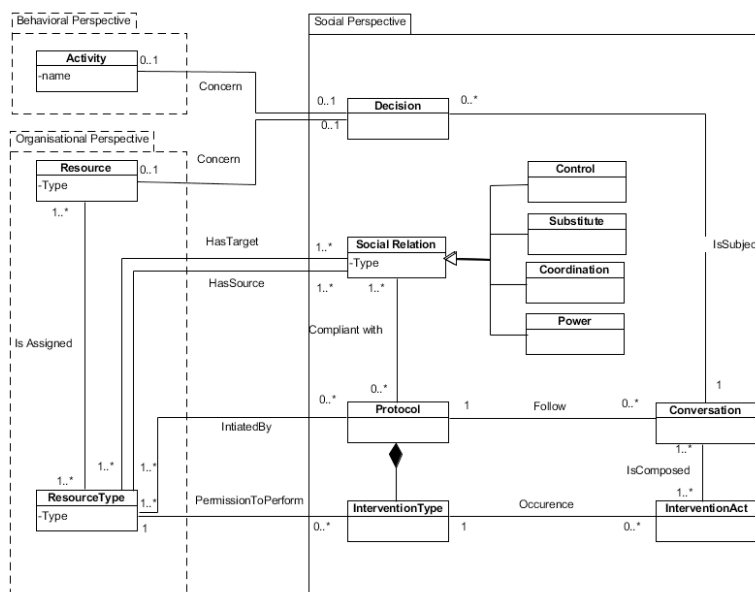
Fig. 4. social perspective
