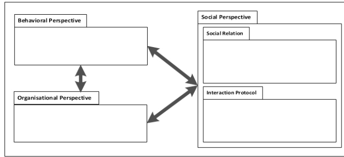
Fig. 1. process perspectives
