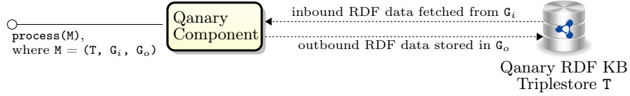
Fig. 1. Qanary Component Model (note that G_i might be equal to G_o ).
