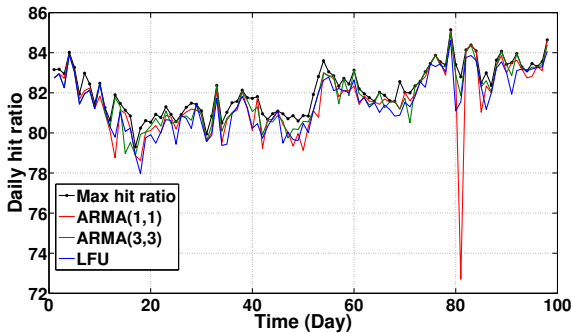
Fig. 8: Zoom on best experts.
