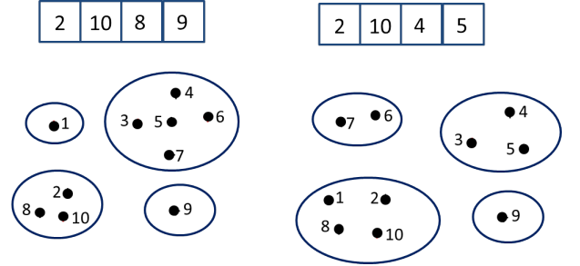
Fig. 8: Impact of the initial random selection in K-means.
