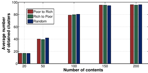
Fig. 2: Average number of clusters.
