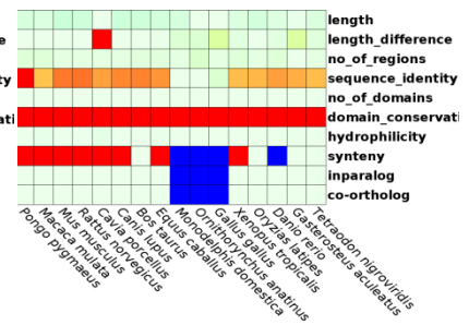
c. Cdk2
