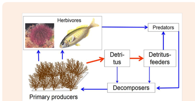
Figure 3: A simplified sketch of food-webs in undisturbed Mediterranean marine benthic ecosystems. Here, a Cystoseira forest. Herbivores are the sea urchin Paracentrotus lividus and the teleost Sarpa salpa . The intensity of the flow is proportional to the width of the arrow between functional compartments (in red, the main path). From Boudouresque et al. (2005) and Boudouresque (2015b), modified.
