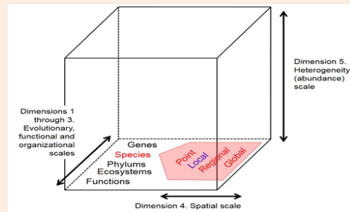
Figure 2: Biodiversity is a multidimensional concept. Dimensions 1 through 3: from genes to ecosystems, landscapes/seascapes and functions. Within each evolutionary, functional and organizational level (e.g. species), dimension 4 (spatial scale), from point to global. Within each spatial level (e.g. local), dimension 5 (proportional distribution), from e.g. very rare to dominant. From Boudouresque, 2014 (modified).
