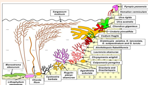
Figure 6: A sketch of the dominant MPOs on shallow (down to 1 m depth) rocky substrates of the Thau Lagoon (southern France) in spring. Most of these taxa are native to Japan, Korea and the northwestern Pacific Ocean (see Figure 7). From Boudouresque et al., 2011, modified.
