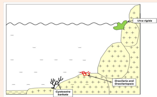
Figure 7: The same sketch as that of figure 6, after the removal of the species native to the northwestern Pacific Ocean. The only native taxa are Cystoseira barbata , Gracilaria sp. and Gracilariopsis sp. Ulva rigida is probably a cryptogenic species (sensu Carlton, 1996). Drawn from data in Boudouresque et al. (2011).
