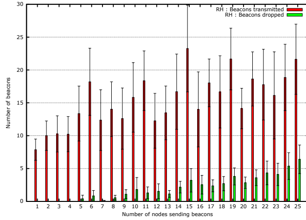
Figure 4: RH: Transmitted vs dropped beacons.
