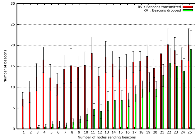
Figure 5: RV: Transmitted vs dropped beacons.
