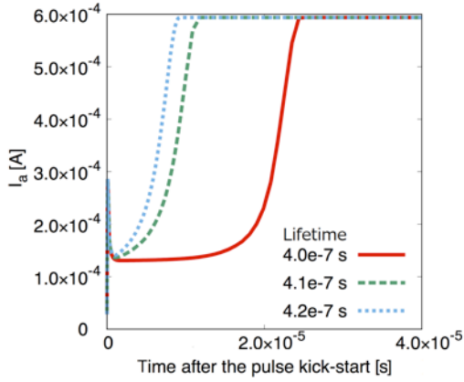
Fig. 6. Simulation result of I_a - t characteristics with variety lifetime. V_{ak} is 300 V. The incident light intensity is 3800 \text{ W/cm}^2 and duration is 0.1 \mu\text{s} . The horizontal axis shows the elapsed time after starting the light irradiation.
