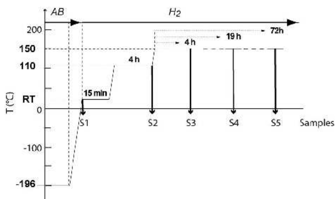
Figure 6: Sketch of the synthesis sequence and samples collected at the different steps, numbered from S1 to S5.
