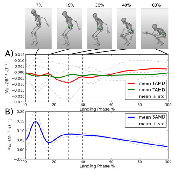
Fig. 2: Mean ( \pm std) of the AMD. In (A, red), the frontal AMD around A-P axis "FAMD". In (A, green), the transversal AMD around vertical axis "TAMD". In (B, blue), sagittal AMD around M-L axis "SAMD". In the top, snapshots of representative configurations extracted from the inverse kinematics computation, of a participant executing the precision landing technique.
