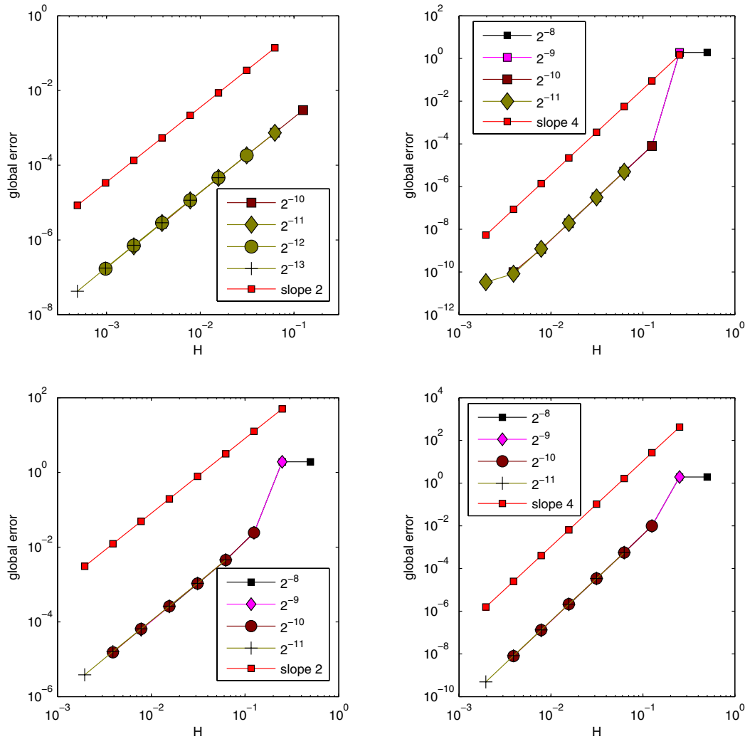
FIGURE 3. Time integration of linear (first row) and nonlinear (second row) test equations (1D) by a second-order (left) and a fourth-order (right) MRCM, respectively, combined with a fourth-order splitting method applied with stepsize h = T_0 \times 10^{-3} . Global errors with respect to numerical reference solutions versus increments H for \epsilon = 2^{-10-j} with j \in \{0, 1, 2, 3\} or \epsilon = 2^{-8-j} with j \in \{0, 1, 2, 3\} , respectively. Reference lines of slopes 2 and 4 are drawn correspondingly. See Table 1.
