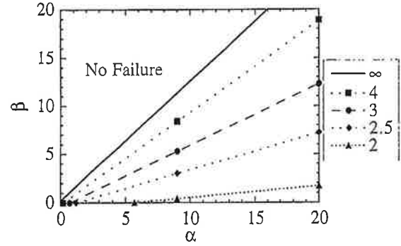
Fig. 9. Fatigue failure maps giving the logarithm of the normalized number of cycles to failure as a function of the parameters \alpha and \beta , for a given cumulative failure probability P_{F0} = 50\% , and a given load level \sigma/S_u = 0.5 , R = 0 , n = 4 , and k = 1/3 .
