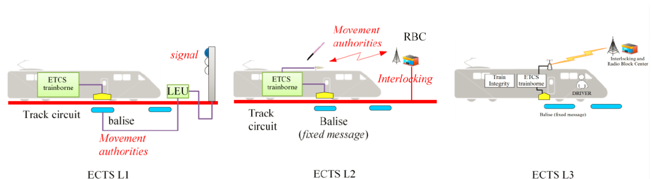
Figure 5: ETCS Levels [4]
