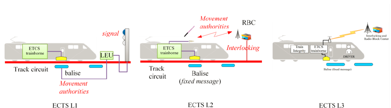
Figure 5: ETCS Levels [4]
