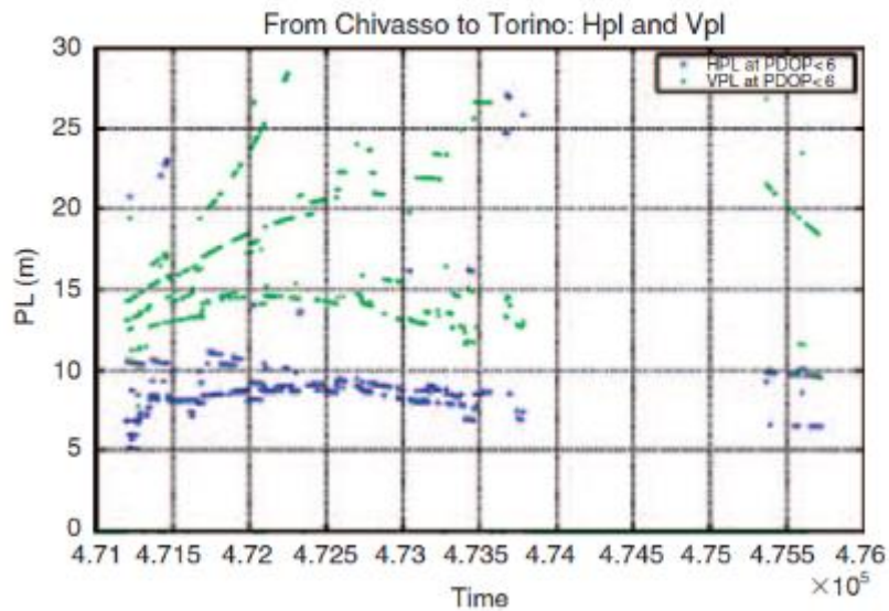
Figure 18: PL obtained in the RUNE project along a line considering that valid positions require that PDOP<6 [18].
