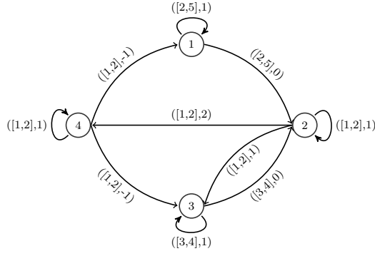
Fig. 5: Associated uniform graph for Example 4.
