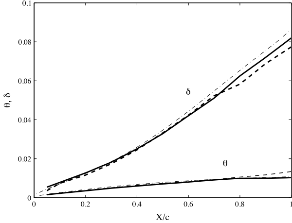
Fig. 5. Mesh convergence study: effect of number of elements and of the confinement on boundary-layer characteristics. (—) fine mesh, order 6, (---) coarse mesh, order 4, (---) XFOIL at a Reynolds number Re = 5000 .
