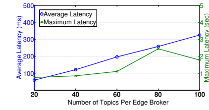
(a) End-to-end Latency of Pub/Sub by Different Number of Topics Per Network
