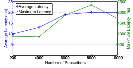
(c) Latency of Coordination Service by Different Number of Joining Subscribers
