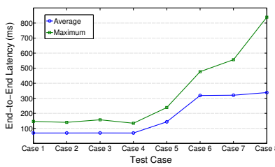
(b) End-to-end Latency of Pub/Sub Multi-path Overlays
