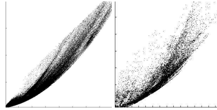
Figure 7. Quantitative results for uncertainty of global models (Old Town on the left, and Small Room on the right). Each patch has coordinates (d_i(P), U_i(P)) with P the representative point of the patch, d_i(P) and U_i(P) the mean depth and the uncertainty ( p = 90\% ) of P by the local model l which reconstructs P . The ranges (cm) are [103, 890] \times [0.63, 39.9] (left) and [55.6, 212] \times [0.72, 7.56] (right), and exclude 0.5% of patches.
