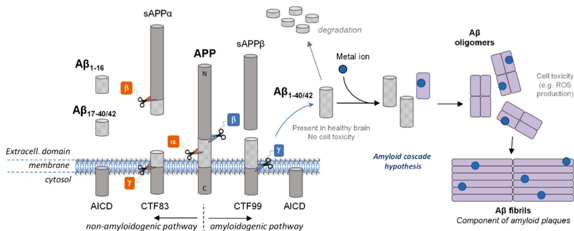
Fig. 1. A schematic view of APP proteolytic cleavage. In the non-amyloidogenic pathway, APP is first cleaved by \alpha -secretase and then by \gamma -secretase to form truncated A\beta_{17-40/42} peptides or by \beta -secretase leading to the formation of the truncated A\beta_{1-16} . In the amyloidogenic pathway, APP is cleaved consecutively by the \beta - and \gamma -secretases leading to the formation of full-length A\beta_{1-40/42} peptides. According to the amyloid cascade hypothesis, the A\beta peptide would be further able to interact with metal ions present in the brain and form oligomers and then fibrils, found in the senile plaques in vivo .
