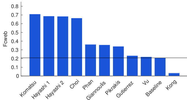
Figure 1: Global performance of the systems submitted to DCASE 2016 - Task 2, in terms of F_{cweb} . Baseline performance is shown with a straight line.
