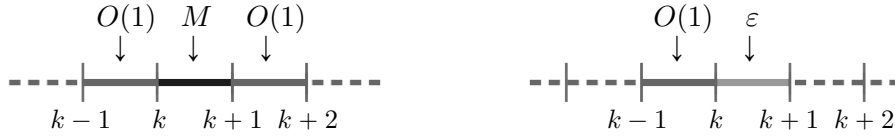
FIGURE 1. On the l.h.s. a trap of the BiRC due to the presence of a large conductance, c_k = M \gg 1 , surrounded by two conductances of O(1) . On the r.h.s. a trap generated by a small conductance c_k = \varepsilon \ll 1 preceded by a conductance of O(1) .
