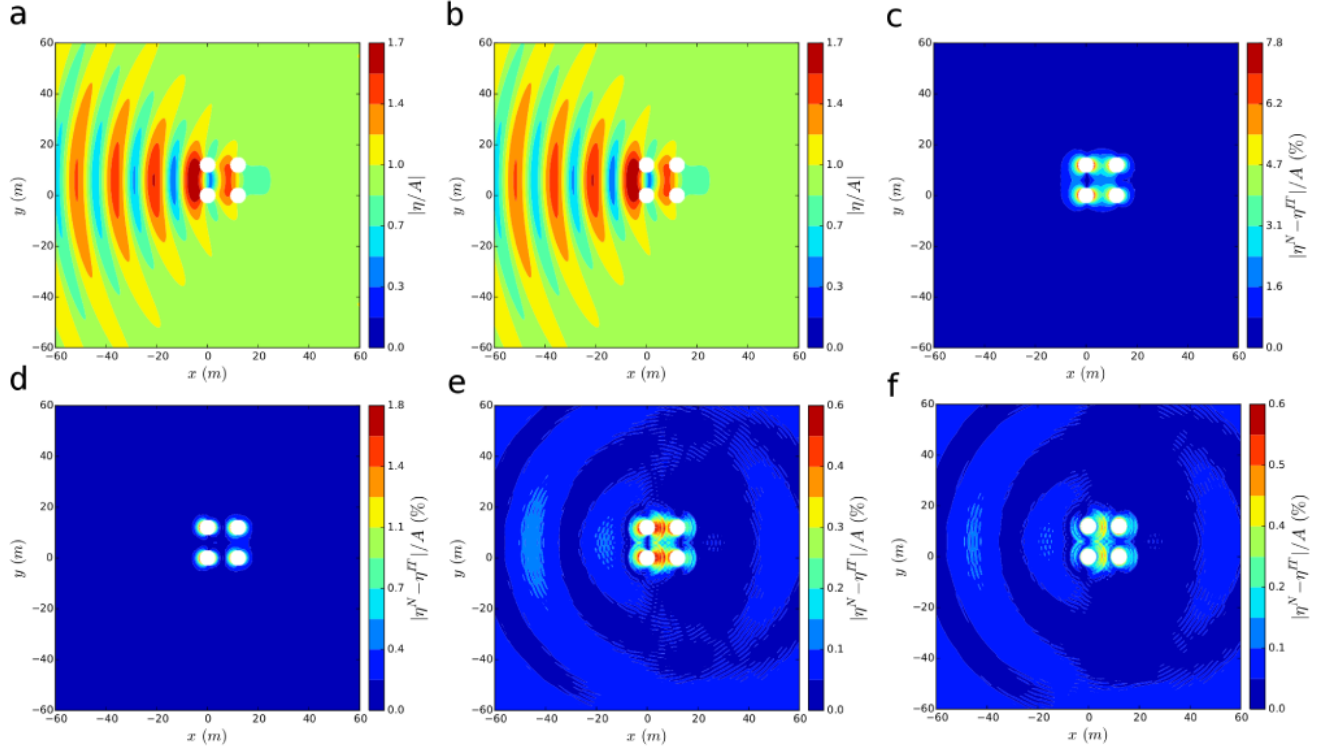
Figure 17: Magnitude of surface elevation for an array of 4 cylinders of radius ( a ), draft ( 2a ) in a water depth ( 50a/3 ) with a separation distance of 4a . Subplot a ) shows the magnitude of the free surface elevation obtained from a direct NEMOH calculation and normalized by the amplitude of the incident wave, subplot b ) shows the same result computed with the interaction theory (IT), and subplots c ), d ), e ), f ) show the percentage difference between the wave fields computed with the interaction theory and the direct NEMOH calculation as a function of the evanescent modes truncation L ( (c) - L = 0 , (d) - L = 6 , (e) - L = 12 , (f) - L = 18 ). Propagation direction is defined from left to right.
