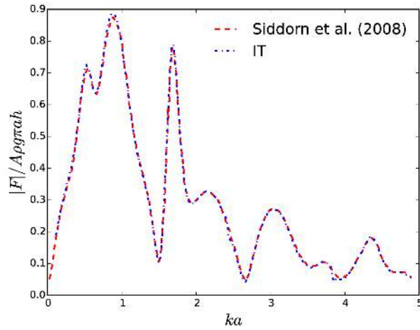
Figure 19: Variation of the surge excitation force on Cylinder 1 (Figure 16) of an array of 4 truncated vertical cylinders with radius ( a ), draft ( h = 2a ) in a water depth of ( 4a ) with each cylinder disposed at the vertex of a square of side size 4a for an incident wave heading angle of \beta = \pi/4 . The nondimensionalization factor terms are the wave amplitude ( A ), the cylinder radius ( a ) and the cylinder draft ( h ).
