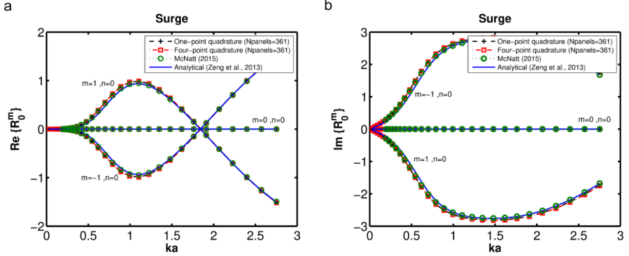
Figure 8: Real and imaginary parts of the Radiation Characteristics progressive terms for a truncated vertical cylinder of 3m radius (a), 6m draft moving in surge in a 10m water depth.
