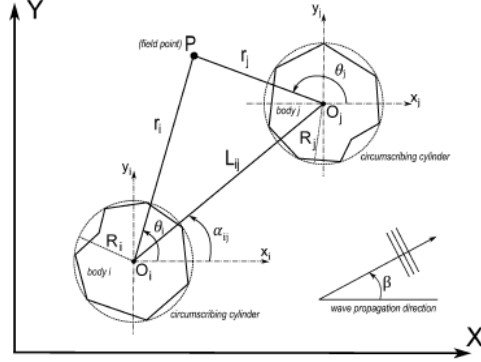
Figure 2: Schematic of the plane view of two bodies of arbitrary geometry with the nomenclature and reference systems used in this paper.
