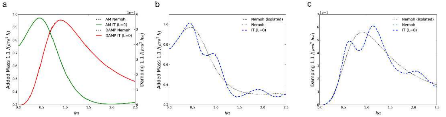
Figure 13: Added mass and damping coefficients for the first truncated vertical cylinder (radius ( a ), draft ( h = 2a ) in a water depth ( 50a/3 ) in the two body array (Figure 12) for different separating distances ( d/a = 5000 - (a), d/a = 5 - (b), d/a = 5 - (c)). First index corresponds to the direction of the force and the second to the degree of freedom.
