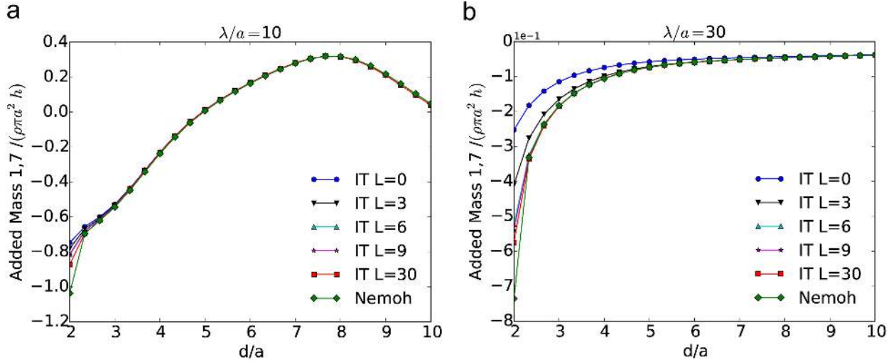
Figure 15: Surge-surge coupling added mass coefficient as a function of the evanescent modes truncation L for two different wavelengths for a small array of two truncated vertical circular cylinders of radius a , draft h = 2a in water depth of 50a/3 .
