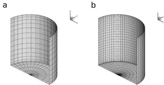
Figure 4: Truncated vertical cylinder mesh. Only half of the geometry is shown due to symmetry. (a) - coarse mesh, 361 panels; (b) - fine mesh 1521 panels.
