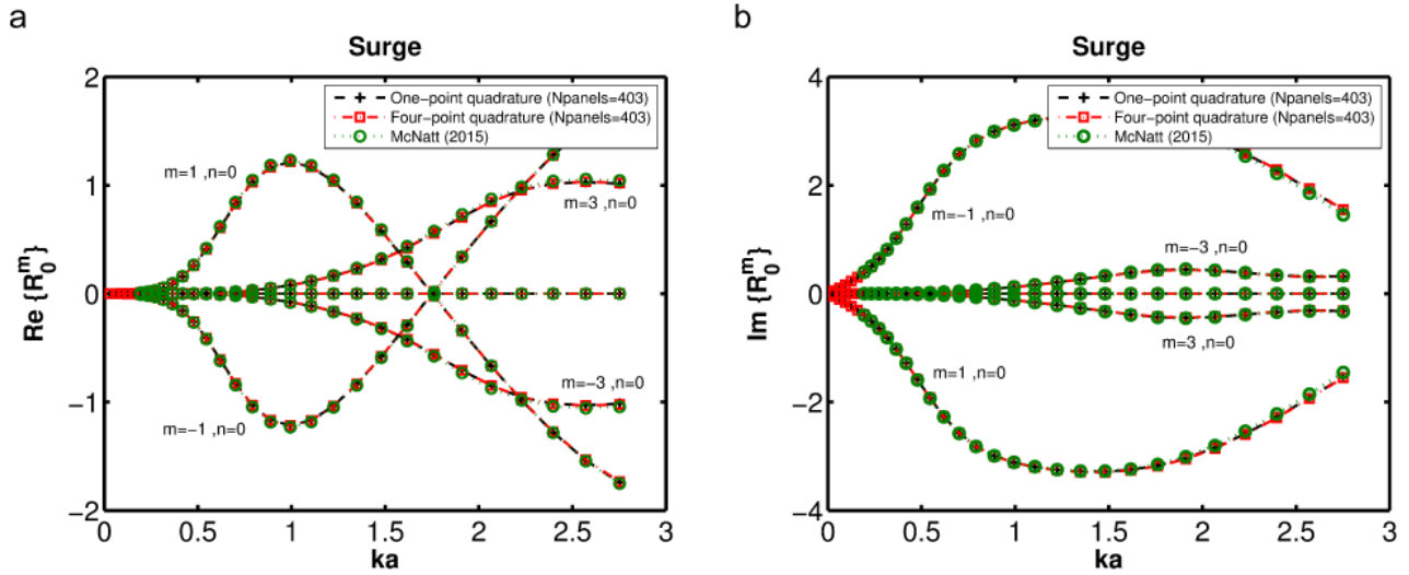
Figure 9: Real and imaginary parts of the Radiation Characteristics progressive terms for a square box of 6m side (2a), 6m draft moving in surge in a 10m water depth.
