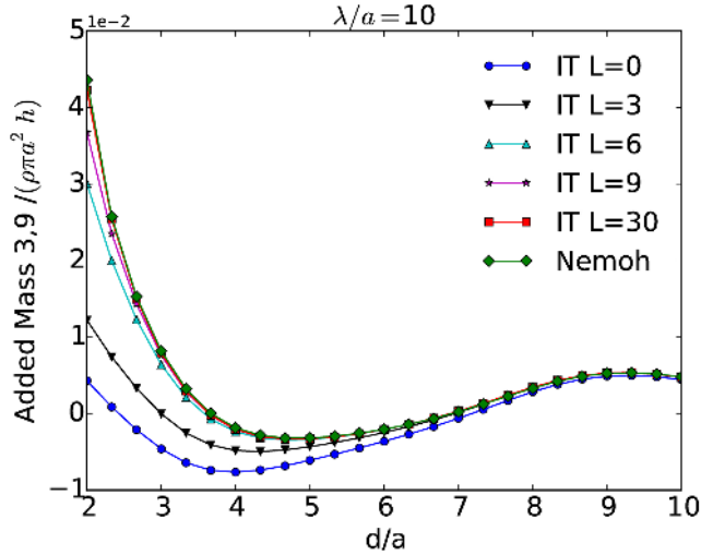
Figure 14: Heave-heave coupling added mass coefficient as a function of the evanescent modes truncation L and for a small array of two truncated vertical circular cylinders of radius a , draft h = 2a in water depth of 50a/3 .
