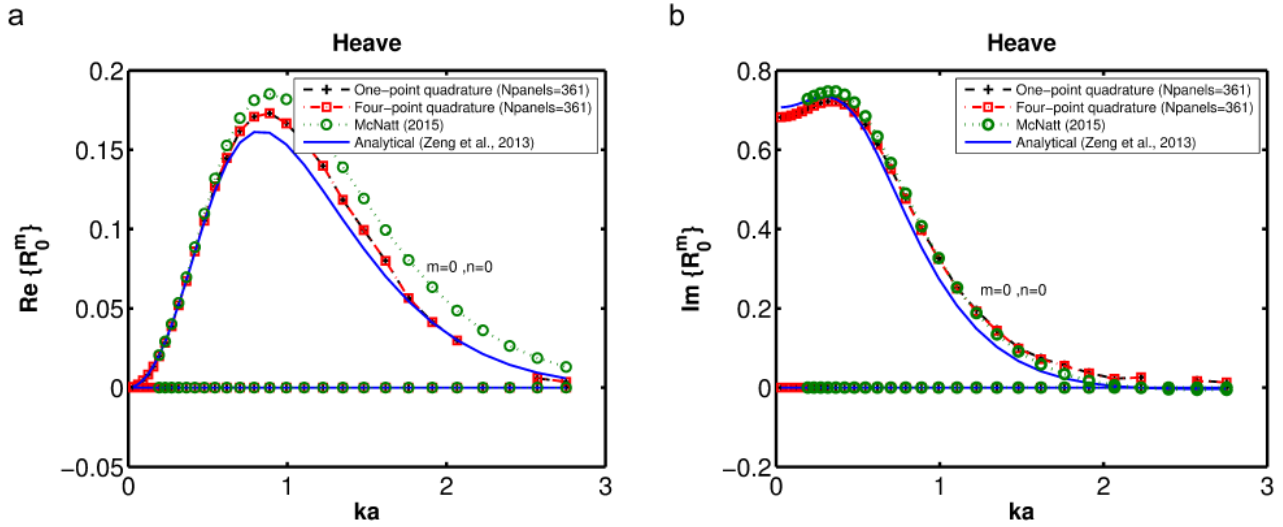
Figure 10: Real and imaginary parts of the Radiation Characteristics progressive terms for a truncated vertical cylinder of 3m radius (a), 6m draft moving in heave in a 10m water depth.
