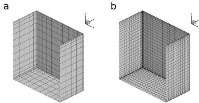
Figure 5: Square box mesh. Only half of the geometry is shown due to symmetry. (a) - coarse mesh, 403 panels; (b) - fine mesh 2059 panels.
