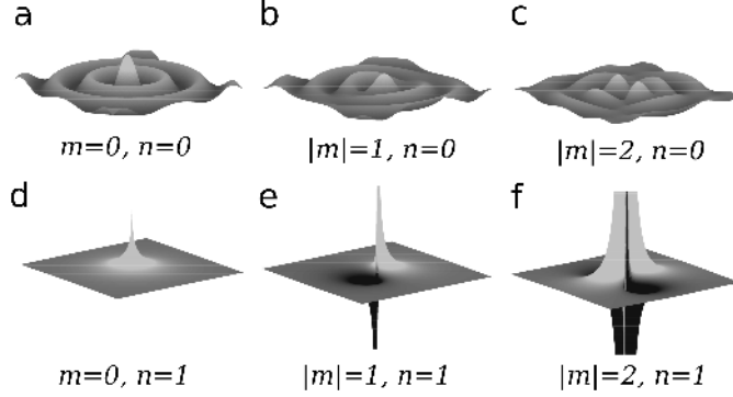
Figure 1: Partial waves modes. Progressive term H_m^{(1)}(r) (a, b, c); evanescent term K_m(r) (d, e, f).
