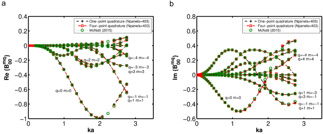
Figure 7: Real and imaginary parts of the Diffraction Transfer Matrix progressive terms for a cube box of 6m side ( 2a ), 6m draft in a 10m water depth.
