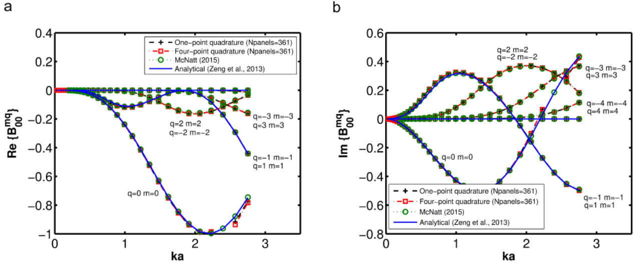
Figure 6: Real and imaginary parts of the Diffraction Transfer Matrix progressive terms for a truncated vertical cylinder of 3m radius (a), 6m draft in a 10m water depth.
