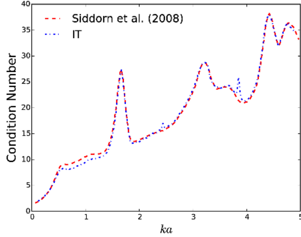
Figure 18: Variation of the condition number (computed using the 1-norm or maximum column-sum) of the scattering matrix of an array of 4 truncated vertical cylinders with radius ( a ), draft ( h = 2a ) in a water depth of ( 4a ) with each cylinder disposed at the vertex of a square of side size 4a (Figure 16).
