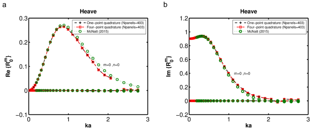
Figure 11: Real and imaginary parts of the Radiation Characteristics progressive terms for a square box of 6m side (2a), 6m draft moving in heave in a 10m water depth.
