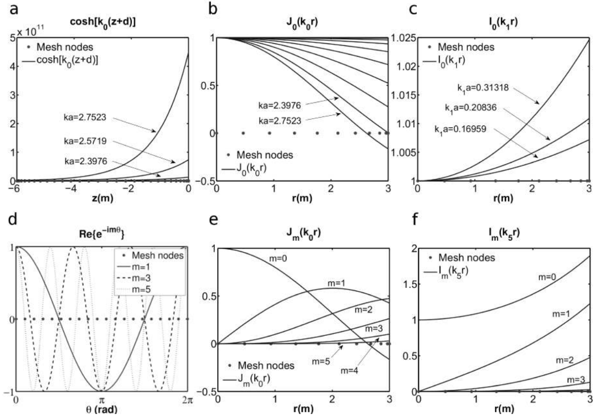
Figure 3: Variation of the hyperbolic cosine depth dependence (a) and angular dependence (d), variation of the Bessel function of the first kind (b, e) and of the modified Bessel function of the first kind (c, f) along the lateral side and the bottom of a cylinder (3m radius, 6m draft in a 30m water depth). Results in (e) are calculated for k_0 a = 2.7523 and in (f) for k_5 a = 1.7279 . The thick points represent the nodes of a given mesh with cosine spacing.
