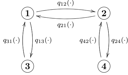
Figure 1: Four-state discrete-time semi-Markov system.
