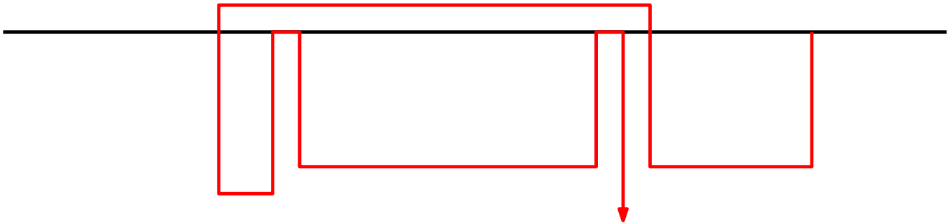
FIGURE 6. The configuration \omega'
