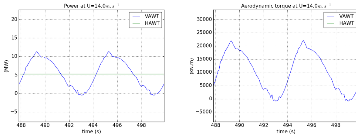
Figure 6: Power and aerodynamic torque acting on the bottom-fixed rotor at U = 14 \text{ m.s}^{-1} .
