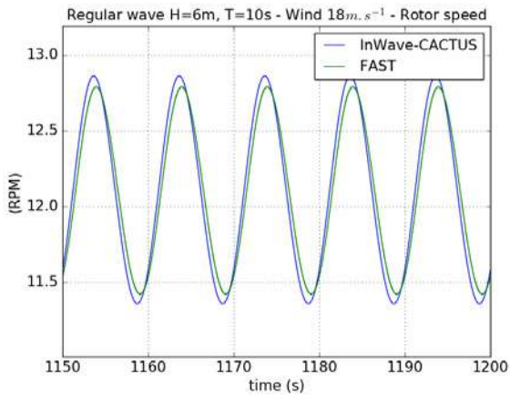
Figure 20: Regular waves and constant 18 \text{ m.s}^{-1} wind – Rotor speed
