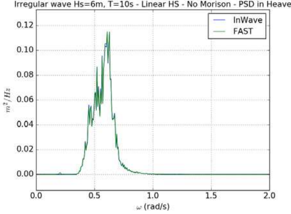
Figure 10: Irregular waves - PSD in Heave
