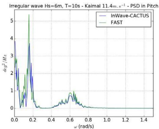
Figure 25: Irregular waves and wind 11.4 \text{ m.s}^{-1} – Pitch PSD
