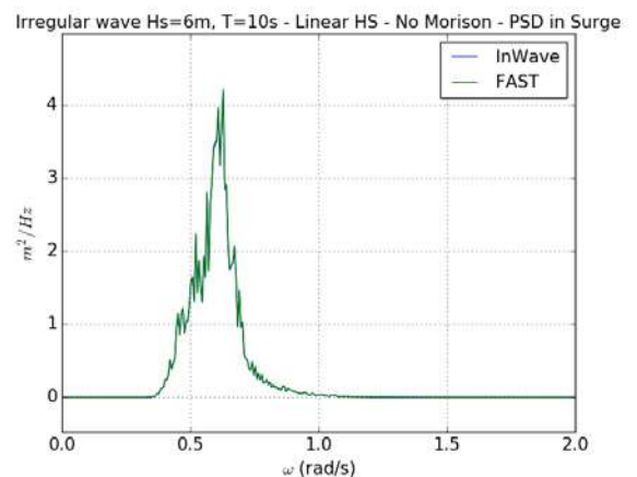
Figure 9: Irregular waves - PSD in Surge
