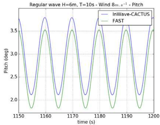
Figure 14: Regular waves and constant 8 \text{ m.s}^{-1} wind – Pitch
