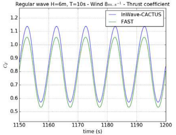
Figure 16: Regular waves and constant 8 \text{ m.s}^{-1} wind – Thrust coefficient
