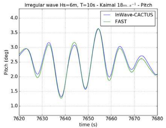
Figure 28: Irregular waves and Kaimal wind U_\infty = 18 \text{ m.s}^{-1} – Pitch
