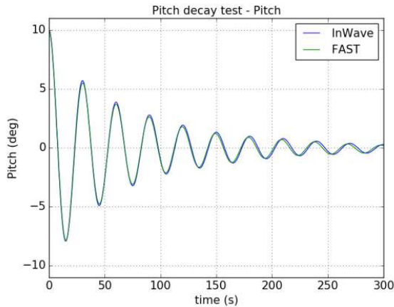
Figure 5: Pitch decay test
