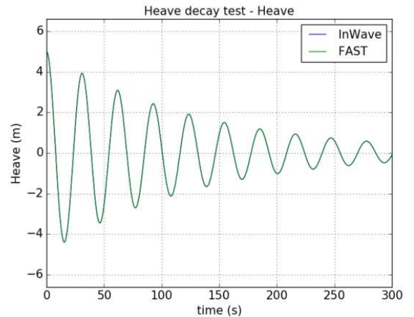
Figure 4: Heave decay test
