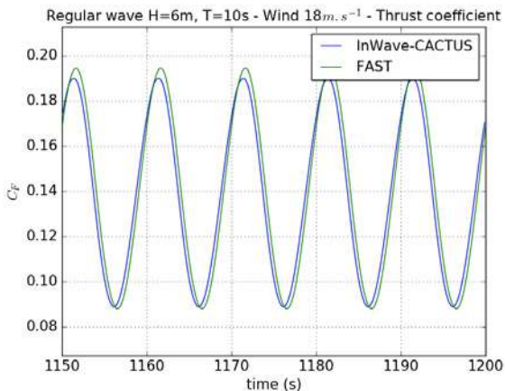
Figure 21: Regular waves and constant 18 \text{ m.s}^{-1} wind – Thrust coefficient
