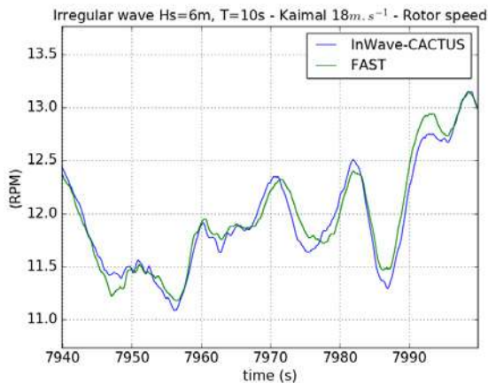
Figure 30: Irregular waves and Kaimal wind U_{\infty} = 18 \text{ m.s}^{-1} – Rotor speed
