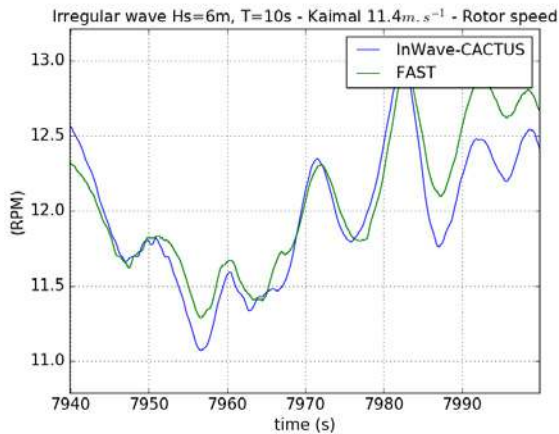
Figure 29: Irregular waves and Kaimal wind U_{\infty} = 11.4 \text{ m.s}^{-1} – Rotor speed
