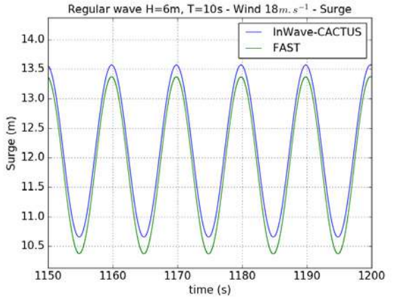
Figure 17: Regular waves and constant 18 \text{ m.s}^{-1} wind – Surge
