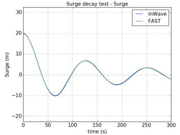
Figure 3: Surge decay test
