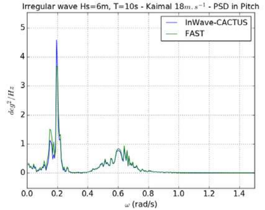
Figure 26: Irregular waves and wind 18 \text{ m.s}^{-1} – Pitch PSD
