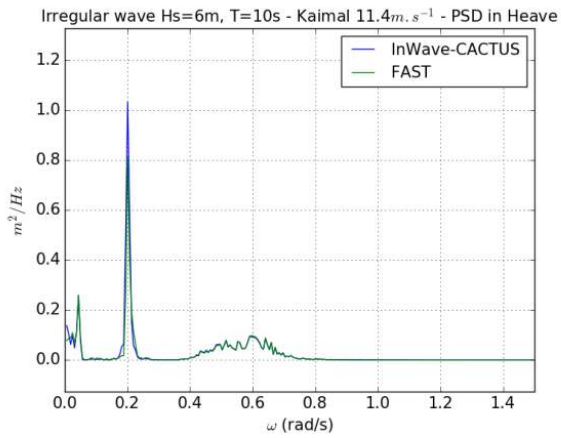
Figure 24: Irregular waves and wind 11.4 \text{ m.s}^{-1} – Heave PSD
