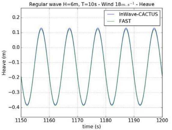
Figure 18: Regular waves and constant 18 \text{ m.s}^{-1} wind – Heave
