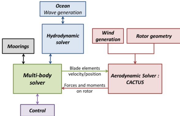
Figure 2: Modular framework coupling InWave and CACTUS
