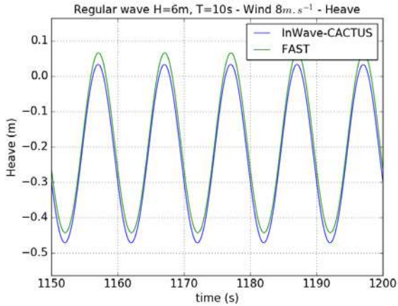
Figure 13: Regular waves and constant 8 \text{ m.s}^{-1} wind – Heave
