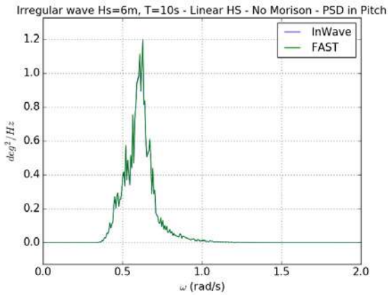
Figure 11: Irregular waves - PSD in Pitch
