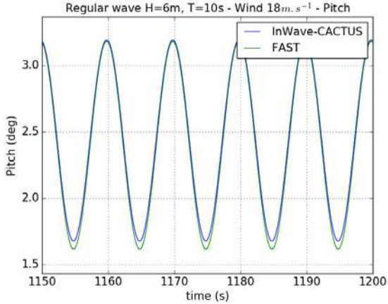
Figure 19: Regular waves and constant 18 \text{ m.s}^{-1} wind – Pitch
