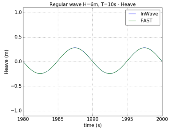
Figure 7: Regular waves – Heave
