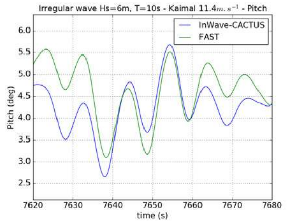
Figure 27: Irregular waves and Kaimal wind U_\infty = 11.4 \text{ m.s}^{-1} – Pitch
