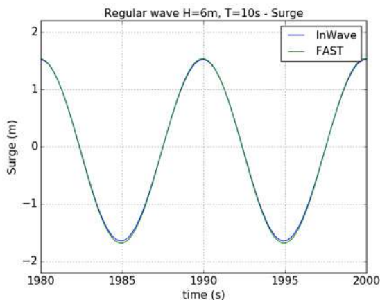
Figure 6: Regular waves - Surge
