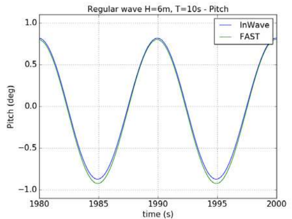
Figure 8: regular waves – Pitch
