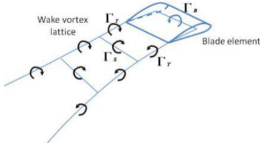
Figure 1: Vortex lattice in free vortex Wake Method from [10]
