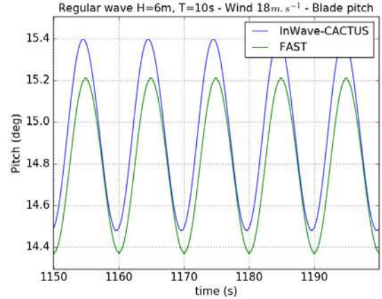
Figure 22: Regular waves and constant 18 \text{ m.s}^{-1} wind – Blade pitch
