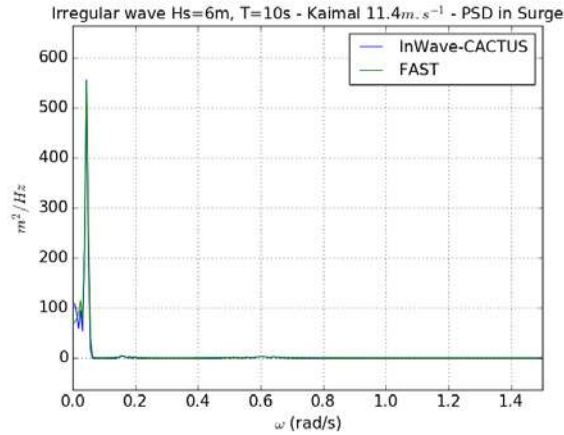
Figure 23: Irregular waves and wind 11.4 \text{ m.s}^{-1} – Surge PSD
