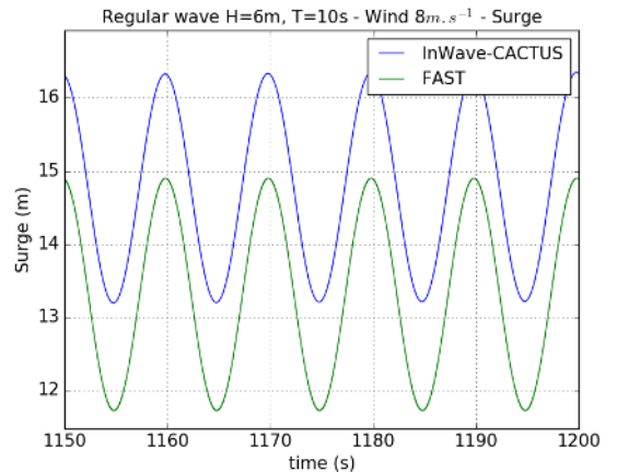
Figure 12: Regular waves and constant 8m.s^{-1} wind - Surge
