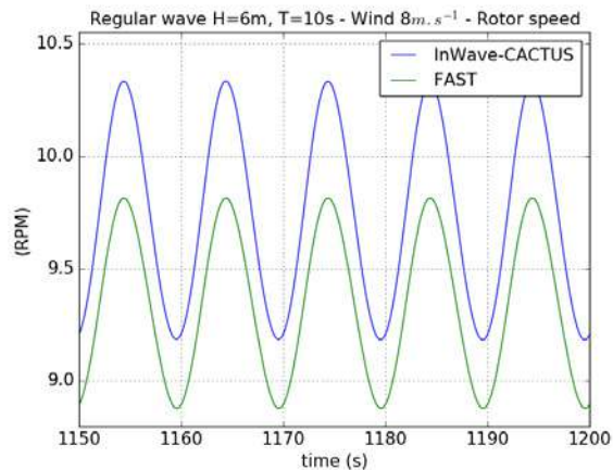
Figure 15: Regular waves and constant 8 \text{ m.s}^{-1} wind – Rotor speed
