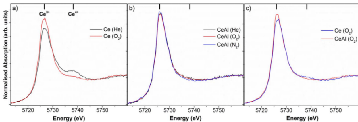
Fig. 3. Normalised Ce L_{m} -edge XANES spectra for Ce-activated silica fiber preforms a) collapsed in He or O_2 ; b) Al codoped preforms collapsed under He, N_2 , or O_2 ; c) Al-free, and Al-codoped preforms collapsed under O_2 .
