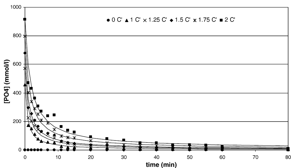
Fig. 2. \text{PO}_4^{3-} in solution during reaction between \text{H}_3\text{PO}_4 and fly ash at 20 °C, 400 rpm, and variable phosphate concentration (C: 453 mmol/l of phosphoric acid).
