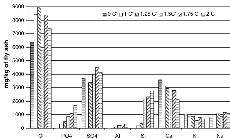
Fig. 10. Major components of fly ash in solution after 80 min reaction between \text{H}_3\text{PO}_4 and fly ash at 20°C, 400 rpm, and variable phosphate concentration (C': 453 mmol/l of phosphoric acid).
