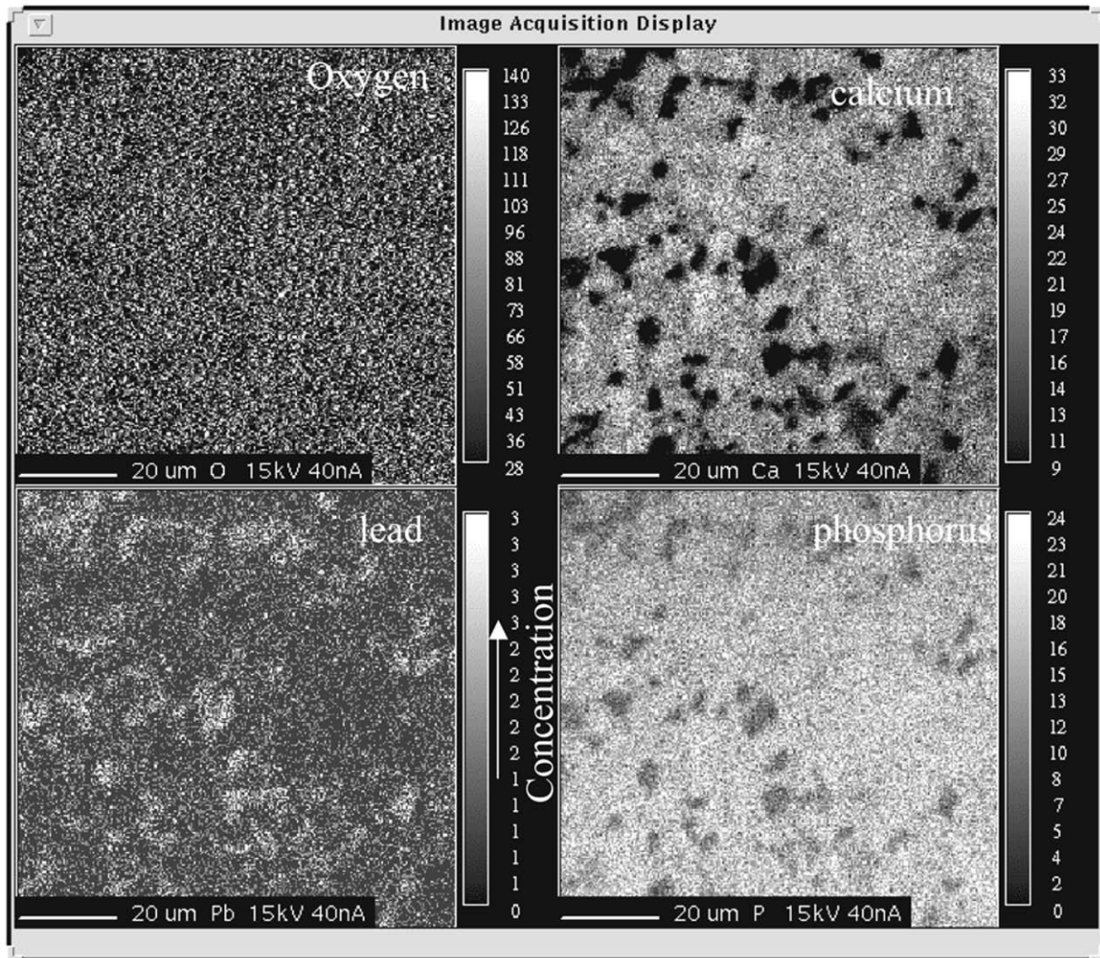
Figure 5. WDS microprobe analysis of the experiment with initial lead concentration of 5000 mg l -1 .
