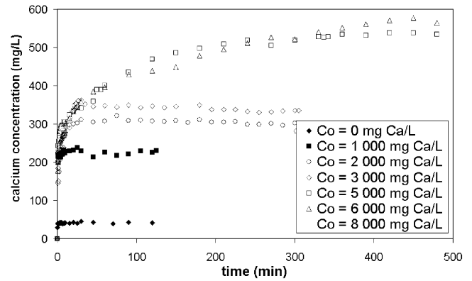
Figure 3. Ca^{2+} released to the solution.
