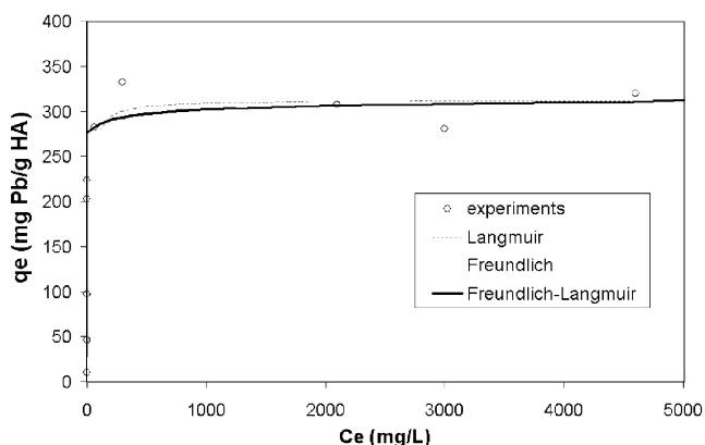
Figure 7. Isotherm ( 25^\circ\text{C} ) of \text{Pb}^{2+} sorption by hydroxyapatite.
