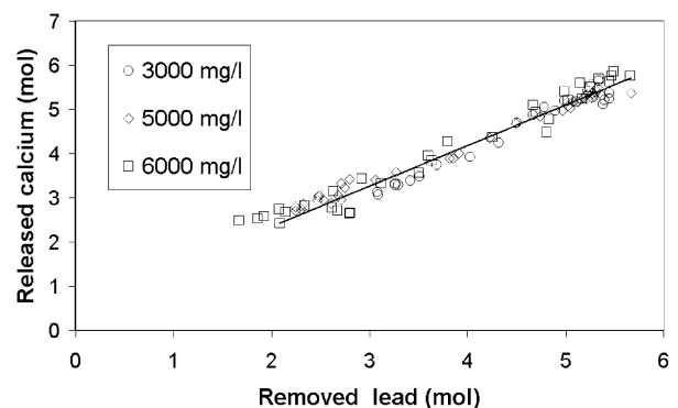
Figure 4. Moles of Ca^{2+} released to the solution as function of moles of Pb^{2+} removed from the solution.
