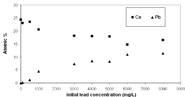
Figure 6. Surface atomic percentage of lead removed and calcium released.
