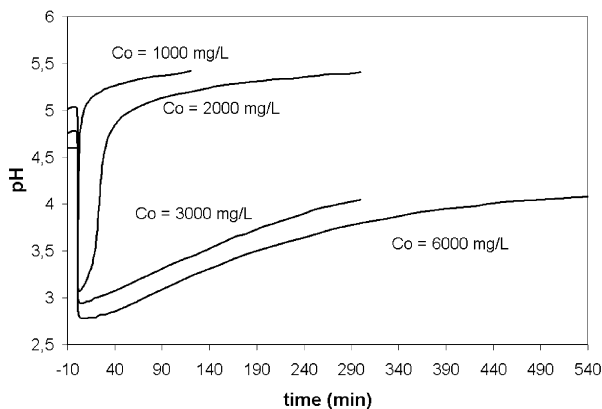
Figure 2. Effect of sorption on the pH of the solution.
