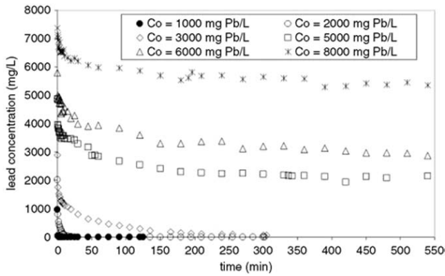
Figure 1. Batch sorption kinetic measurements.
