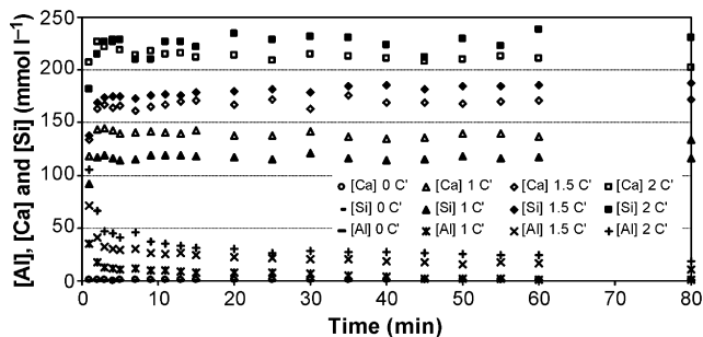
Figure 12. \text{Al}^{3+} , \text{Ca}^{2+} and \text{Si}^{4-} in solution during reaction between \text{H}_3\text{PO}_4 and melilite at 20^\circ\text{C} and 400 rpm. C: 453 \text{ mmol l}^{-1} of phosphoric acid.
