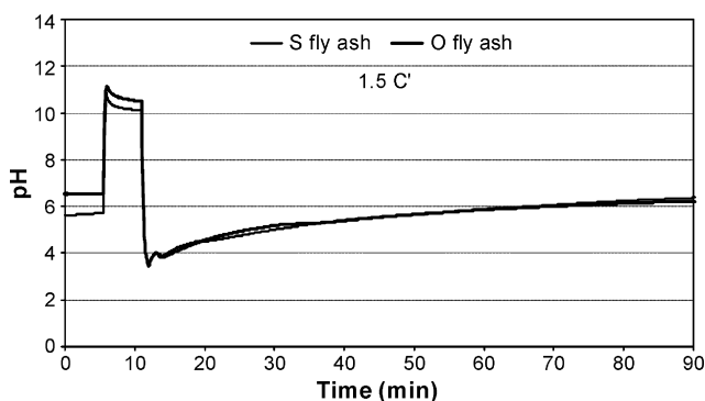
Figure 1. pH of the suspension during reaction between H 3 PO 4 and fly ashes at 20^\circ\text{C} , 400 rpm and phosphate concentration of 1.5 C' . C' : 453 \text{ mmol l}^{-1} of phosphoric acid.
