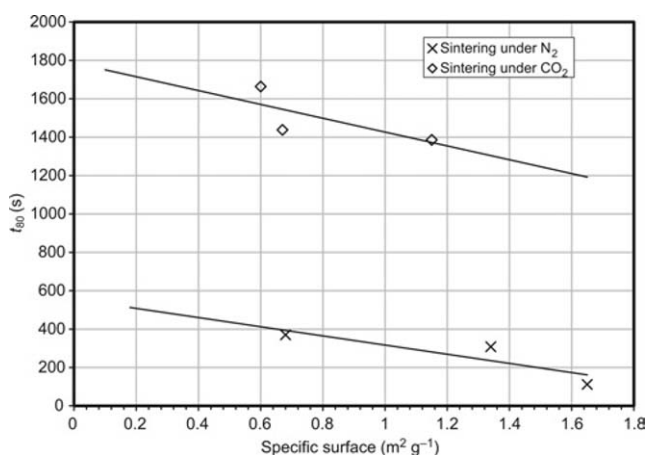
Figure 8. Time to reach 80% of the final hydration temperature increase ( t_{80} ) versus specific surface after sintering at different temperature under N_2 and under CO_2 atmosphere.
