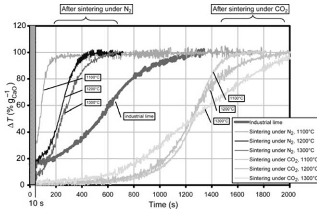
Figure 7. Hydration activity of lime sintered under N_2 and CO_2 ; hydration activity and industrial lime produced in packed-bed.
