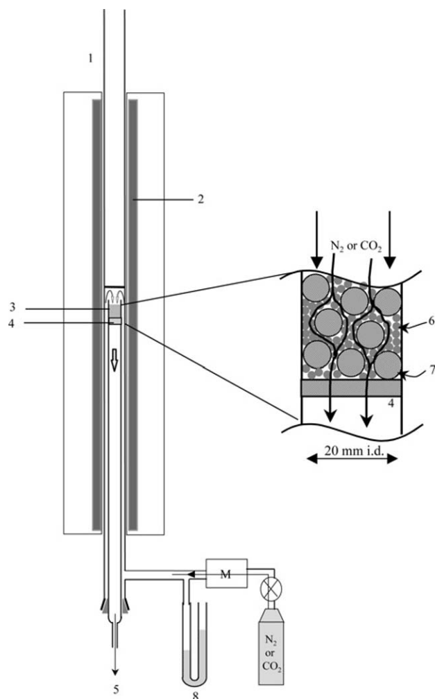
Figure 1. Crossed fixed bed. (1) Quartz tube; (2) electrical heater; (3) particles bed; (4) filtering sheet; (5) exhaust gases; (6) lime particles; (7) ruby balls; (8) water column manometer; M—mass flow meter/controller; \text{N}_2 —nitrogen; \text{CO}_2 —carbon dioxide.
