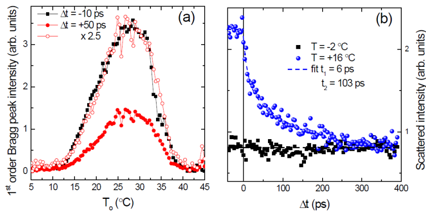
Figure 7. (a) 1st order Bragg peak intensity as a function of T_0 for \Delta t = -10 ps (black squares) and \Delta t = +50 ps (red filled circles). For better comparison, the latter is also plotted multiplied by a factor of 2.5 (red open circles); (b) Scattered intensity at the 1st order Bragg peak position as a function of \Delta t for T_0 = -2 °C (no stripes) and T_0 = +16 °C. The dashed blue line is a double exponential decay fit.
