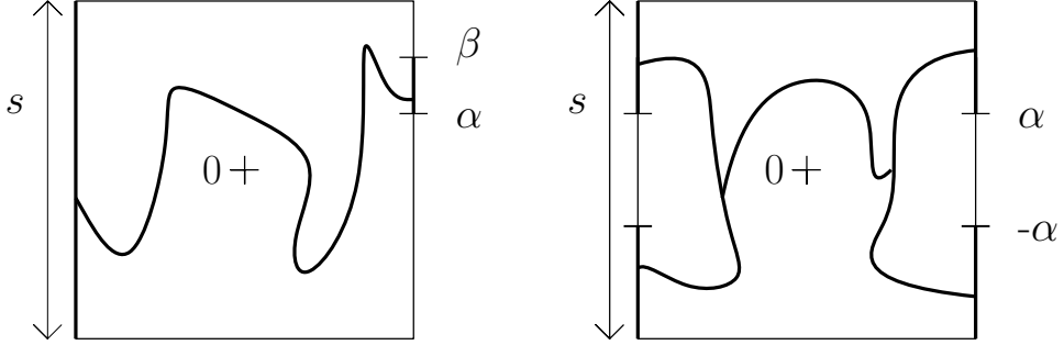
Figure 4: The events \mathcal{H}_s(\alpha, \beta) (left-hand-side) and \mathcal{X}_s(\alpha) (right-hand-side). For every \alpha \in [0, s/2] , we let \phi_s(\alpha) = \mathbb{P}[\mathcal{H}_s(0, \alpha)] - \mathbb{P}[\mathcal{H}_s(\alpha, s/2)] .
