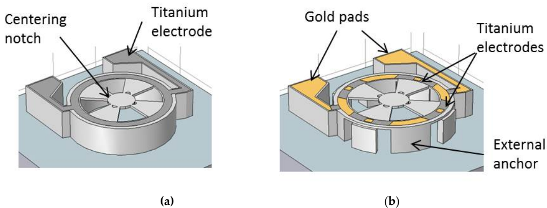
Figure 2: (a) Previous design of the electro thermally-actuated polymer-based MOEMS already including centering notches for lens positioning (b) New design including localized heating areas and external anchors
