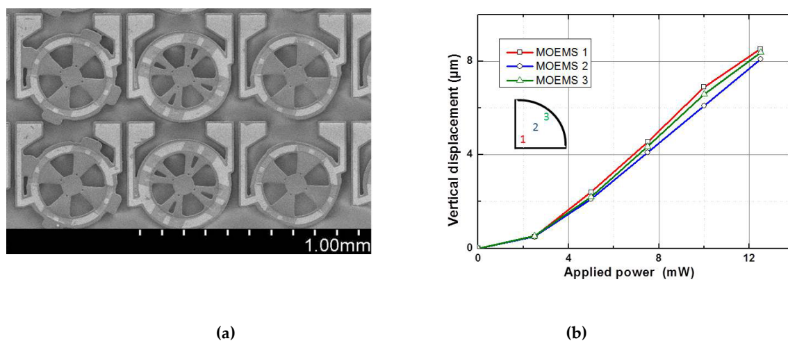
Figure 4: (a) SEM (Scanning Electron Microscopy) view of a DF-1050 MOEMS arrays with different tested designs (b) Vertical displacement of the membrane for MOEMS located in different arrays of the GaAs sample and comparison with modeling.
