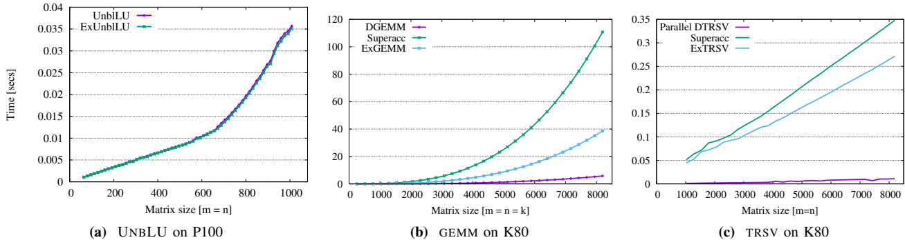
Figure 2: Performance results.
