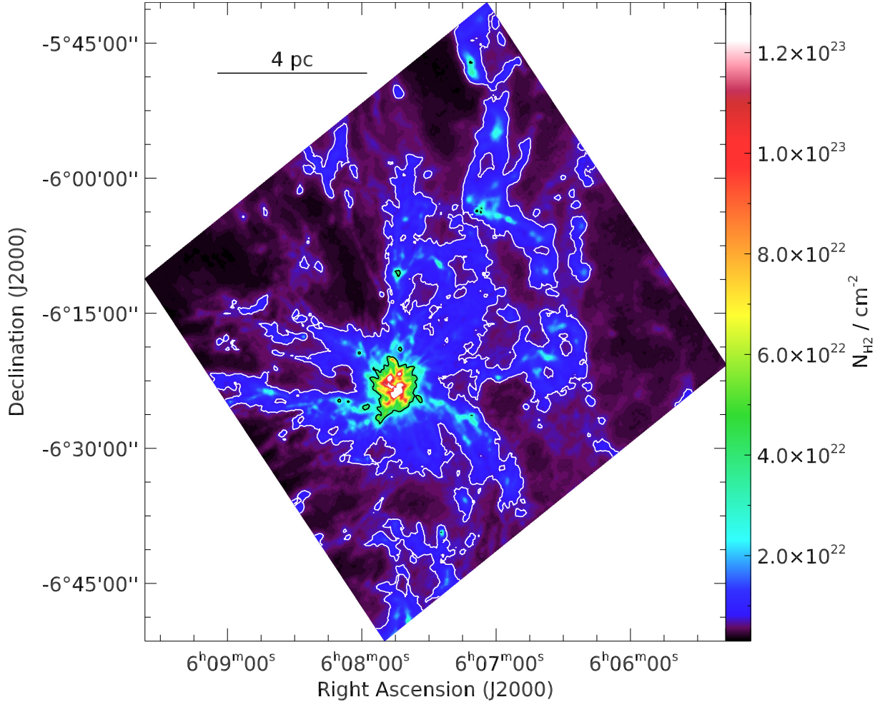
Fig. 3. Monoceros R2 high-resolution \text{H}_2 column density map ( \tilde{\Sigma} ). The resolution is as for the 250\ \mu\text{m} map ( 18.1'' ). The contours are at the \text{H}_2 column densities 7.5 \times 10^{21}\ \text{cm}^{-2} (white) and 3.5 \times 10^{22}\ \text{cm}^{-2} (black).
