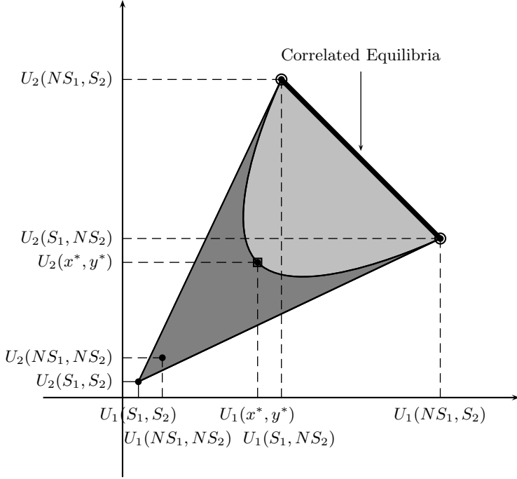
Figure 3: The Correlated Equilibria.
