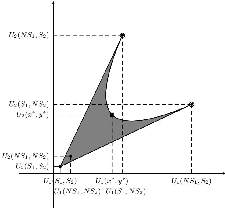
Figure 2: The Equilibrium and Feasible Utilities.
