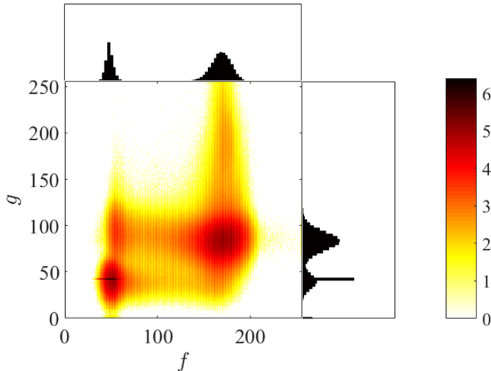
Figure 2. \log_{10} -scale joint histogram of gray levels from the sections shown in Fig. 1 with no registration. f(\mathbf{x}) is the x-ray image, and g(\mathbf{x}) is the neutron image. Histograms of each individual image are presented in black on a linear scale.
