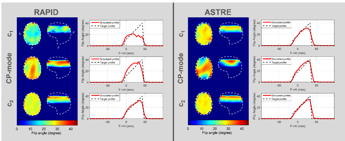
Figure 3: Flip angle Bloch simulations for 3-spoke excitations following c1 and c2 designs, and for the standard circularly polarized (CP) mode (TBW=10). As for c2, the CP-mode was performed using a ramp excitation waveform. Axial and sagittal flip angle maps and associated slab profiles are shown at the center of the slab of interest.
