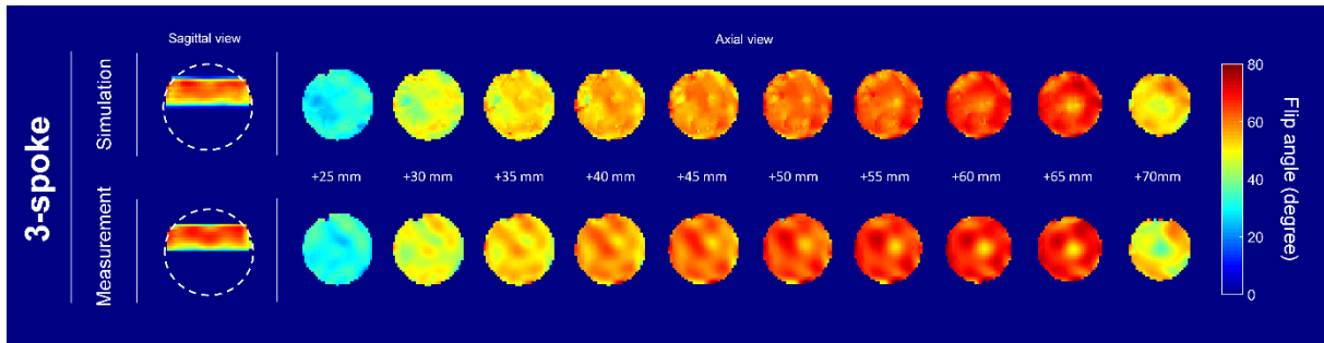
Figure 1: Agreement between FA simulation and measurements with 3-spoke excitations targeting FA=45° to 75° in a 50-mm slab of a spherical water phantom using the ASTRE coil: this validates the simulations performed in this study.
