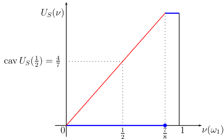
Figure 2: Concavification.
