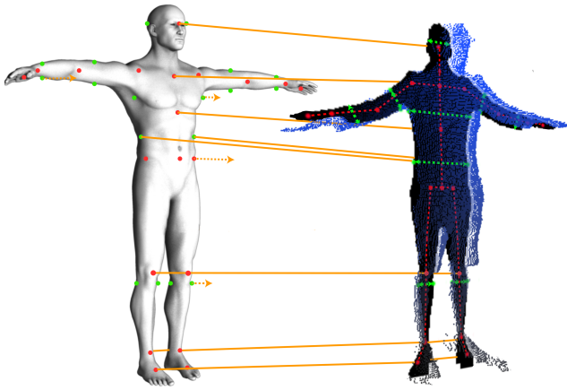
Fig. 4. Skin registration. Red dots: origins of control frames; green dots: silhouette key points; blue dots: Kinect point cloud.
