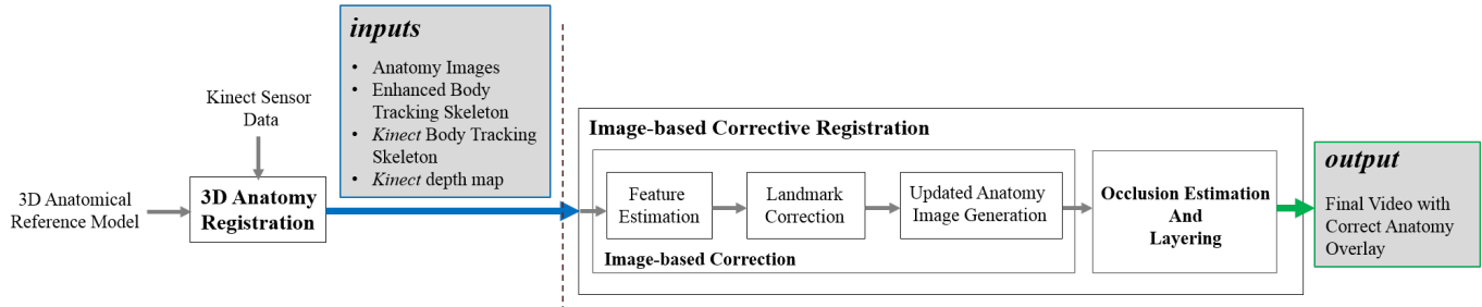
Fig. 17. Overview of our corrective registration system.
