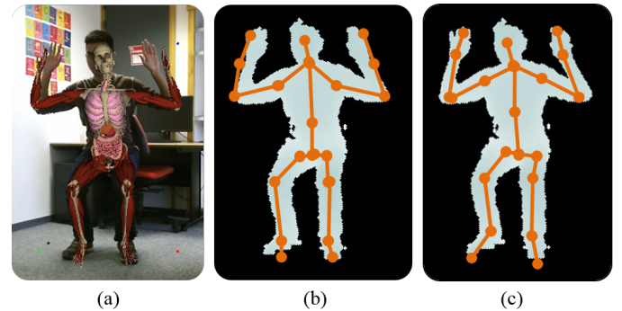
Fig. 20. Landmark correction: Our skeleton correction algorithm corrects initial Kinect 2D skeleton in image space (b) to produce more consistent configurations (c).
