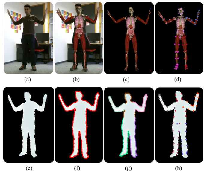
Fig. 19. Feature estimation: Preliminary 3D registration when superimposed on input image (a) we can observe anatomy misalignments (b). We estimate anatomy features (d) from the intermediate anatomy images (c). In the bottom row, we show the estimation (f) and segmentation (g) of depth contours from the depth map (e), and estimated depth features (h).
