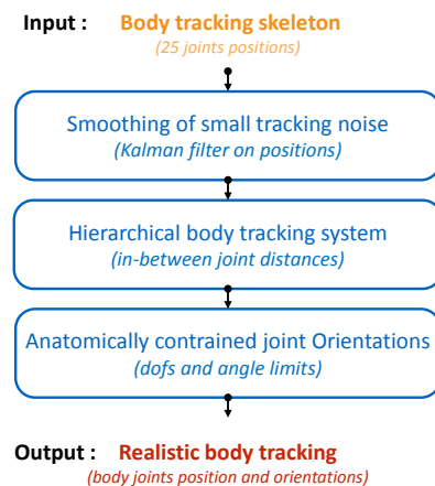
Fig. 9. Enhanced body tracking pipeline.
