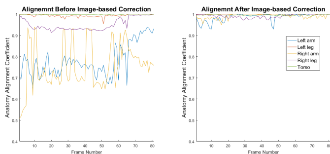
Fig. 24. The anatomy alignment coefficients for anatomy regions are shown before and after image-based correction for the squat sequence.
