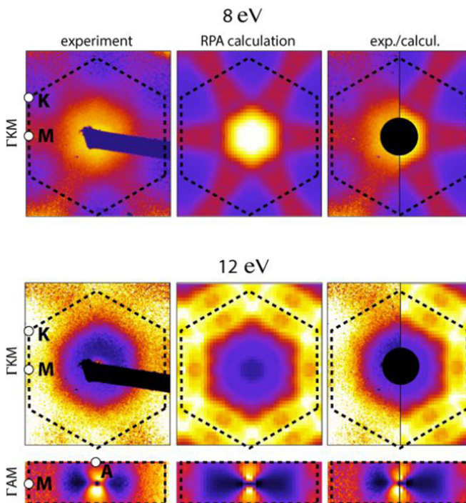
FIG. 8. Experimental and calculated loss functions (scattered intensities multiplied by q^2 ) at 8 eV for the \Gamma KM plane and at 12 eV for the \Gamma KM and \Gamma AM planes. Dashed lines delimit the Brillouin zone.
