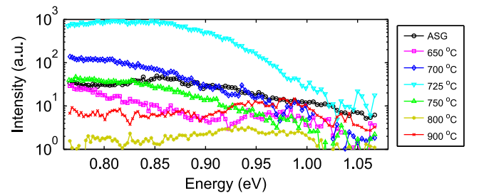
Fig. 2. Time-integrated ( 0 \leq t \leq 600 \mu\text{s} ) PL spectra (please note the log scale on the vertical axis), obtained from samples annealed at different temperatures and excited by a pump fluence of \approx 8 \cdot 10^{-6} \text{ J/cm}^2 at a sample temperature of 16 K.
