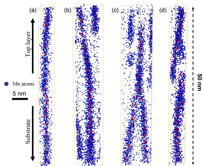
FIG. 5. 3D images of single Mn-rich nanocolumns (only the Mn are represented for clarity). (a) Continuous nanocolumn, (b) curved nanocolumn correlated to the nucleation and growth of another nanocolumn, (c) junctions between bent nanocolumns followed by an interruption, (d) discontinuous nanocolumn.
