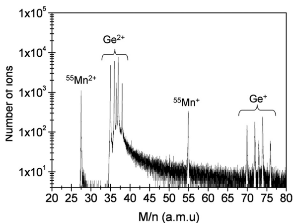
FIG. 3. Mass spectrum of the \text{Ge}_{0.9}\text{Mn}_{0.1} thin film obtained by LAWATAP ( \lambda = 342 nm).
