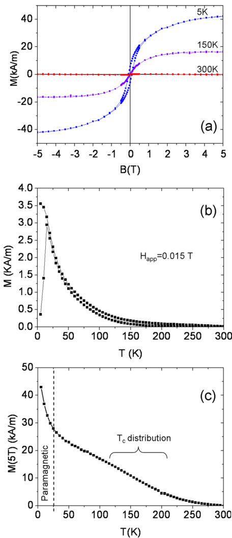
FIG. 10. (a) Hysteresis loops M(H) at 5, 150, and 300 K. (b) ZFC/FC measurements recorded with a field of 0.015 T. (c) Temperature dependence of the magnetization at 5 T ( M_{5T} ). The magnetic field was applied in the film plane.
