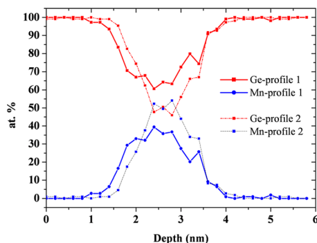
FIG. 9. Corrected concentration profiles taken across a single Mn-rich nanocolumn at two different heights.
