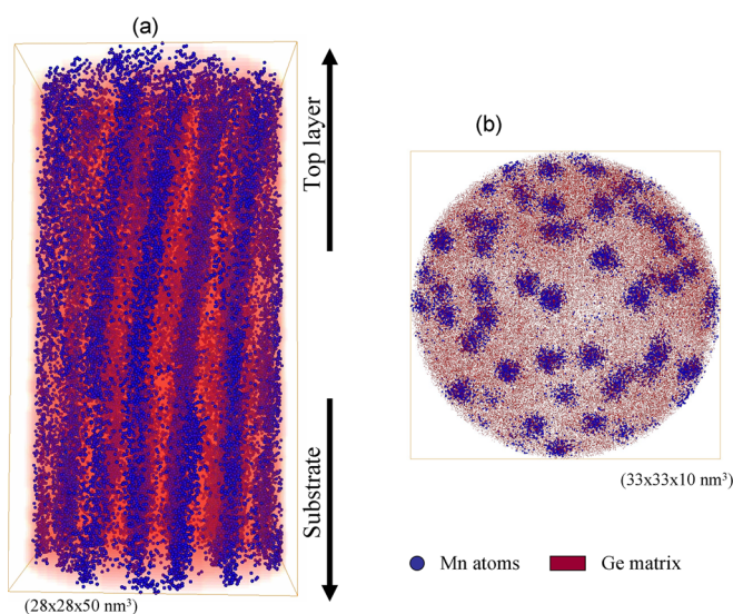
FIG. 4. 3D images of Mn-rich nanocolumns embedded in the Ge matrix obtained by atom probe tomography. (a) Side view, (b) top view. The Mn atoms and the Ge matrix are represented in blue and red, respectively.
