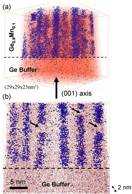
FIG. 7. (a) 3D images of the interface between the Ge buffer layer and the \text{Ge}_{0.9}\text{Mn}_{0.1} thin film. (b) Slice of 2 nm thick taken in the 3D volume showing the interface between the Ge buffer layer and the \text{Ge}_{0.9}\text{Mn}_{0.1} thin film; black arrows indicate the interruption of some nanocolumns. The Mn atoms and the Ge matrix are represented in blue and red, respectively.
